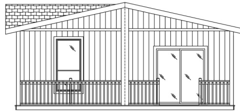
FRONT ENDWALL (W/OPT 8'-0" PORCH)
